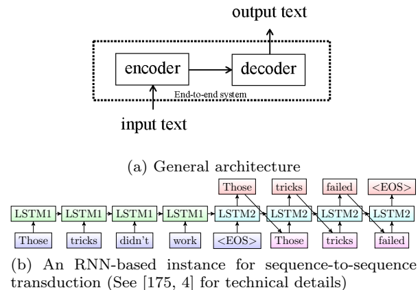
Fig. 5: Encoder-decoder architecture
