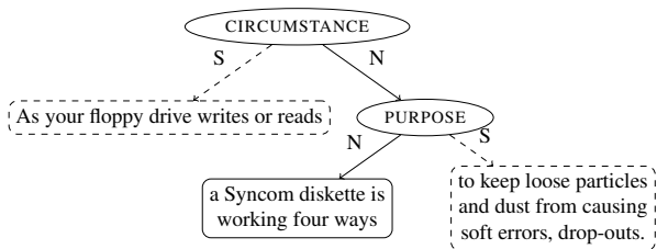
Fig. 3: (An example from [130]) An RST discourse tree with EDUs as leaf nodes
